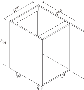
Single Sink Cabinet H: 715 MM W: 600 MM D: 560 MM
