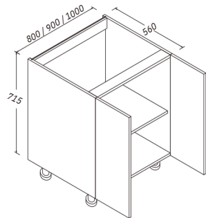
Dual Cabinet H: 715 MM W: 800, 900, 1000MM D: 560 MM
