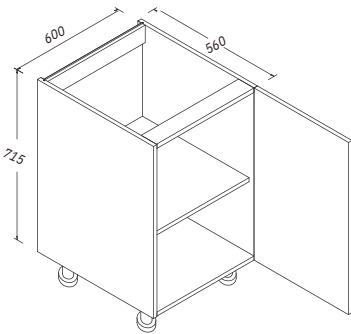
Single Cabinet H: 715 MM W: 600 MM D: 560 MM
