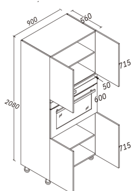
Dual Appliance Column
