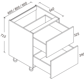
Two Drawer Cabinet H: 715 MM W: 600, 800, 900 MM D: 560 MM
