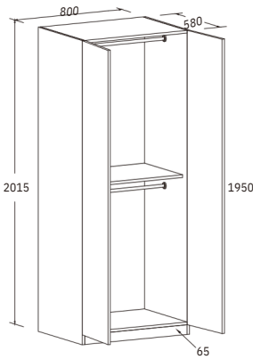
Dual Wardrobe w/ Hangers H: 2015 MM W: 800 MM D: 580 MM
