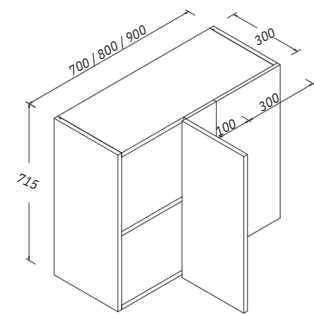
Blind Corner Cabinet H: 715 MM W: 700, 800, 900 MM D: 300 MM
