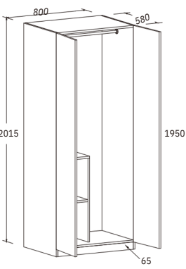
Dual Wardrobe w/Mixed Shelving
