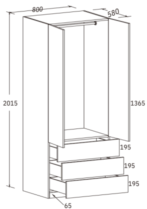
Dual Wardrobe w/Drawers
