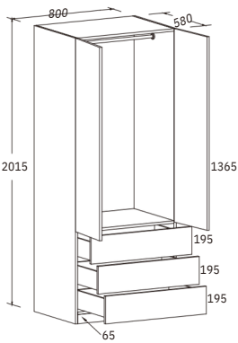
Dual Wardrobe w/Drawers
