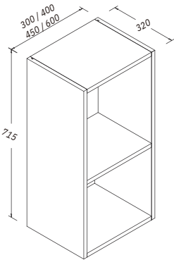
Open Cabinet H: 715 MM W: 300, 400, 450, 600 MM D: 320 MM
