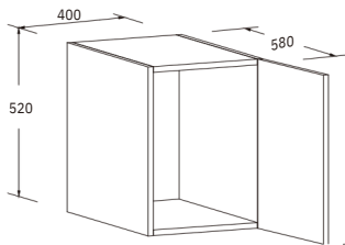
Single Wall Cabinet H: 520MM W: 400 MM D: 580 MM
