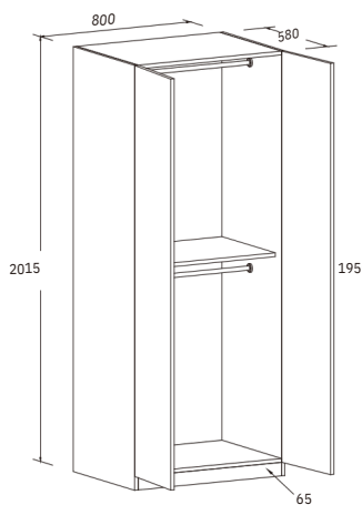
Dual Wardrobe w/Hangers
