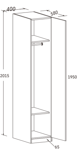
Single Wardrobe w/ Mixed Shelving H: 2015 MM W: 400 MM D: 580 MM
