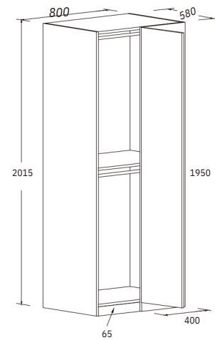
Wardrobe With Corner H: 2015 MM W: 800 MM D: 580 MM
