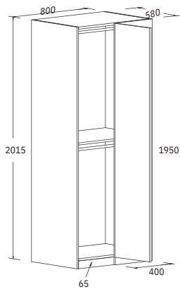
Wardrobe With Corner
