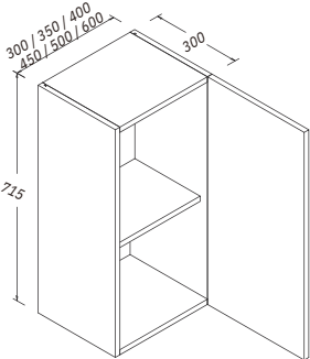
Single Wall Cabinet H: 715 MM W: 300, 350, 400, 450, 500, 600 MM D: 300 MM
