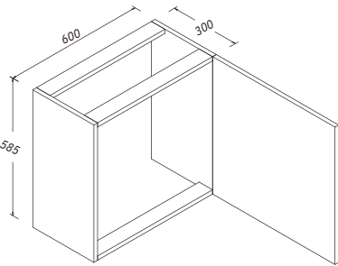
Single Range Hood Wall Cabinet H: 585 MM W: 600 MM D: 300 MM
