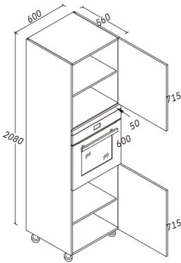
Appliance Column H: 2080 MM W: 600 MM D: 560 MM
