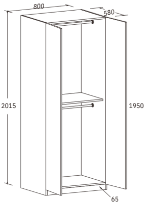
Dual Wardrobe w/ Hangers
