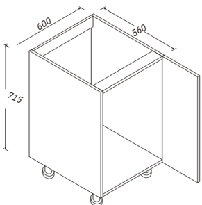
Single Sink Cabinet
