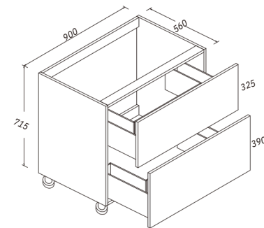
Cooker Cabinet H: 715 MM W: 900 MM D: 560 MM
