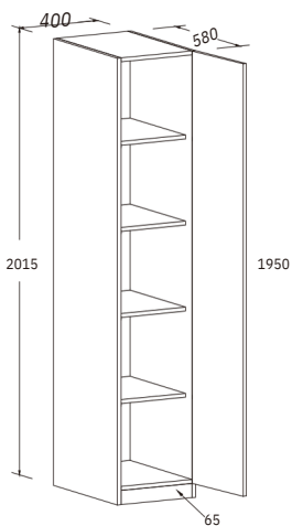
Single Wardrobe w/Shelving H: 2015 MM W: 400 MM D: 580 MM
