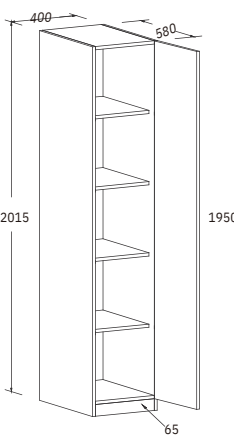
Single Wardrobe w/Shelving
