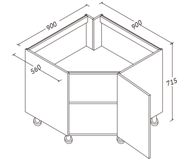
Curved Corner Cabinet H: 715 MM W: 900 MM D: 900MM
