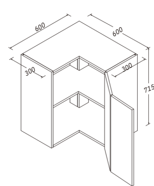
Corner Wall Cabinet H: 715 MM W: 600 MM D: 600 MM
