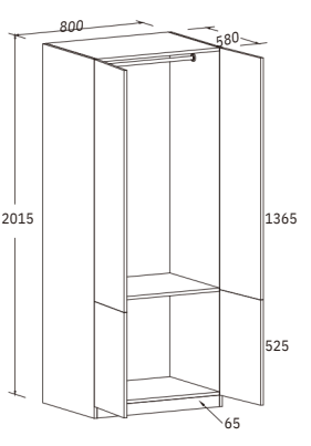
Double-Door Wardrobe H: 2015 MM W: 800 MM D: 580 MM
